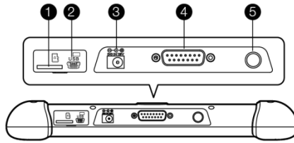
Figure 2-3 MaxiSys MS906 Tablet Top View
